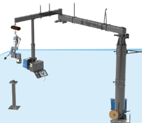
Boom Remote Mounting
