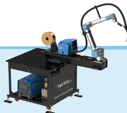
Park'N'Arc Rotational Range Extender
